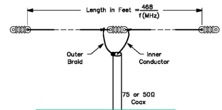
Dipole Antenna
